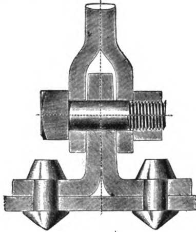
FIG. 113.—CORRECT CONSTRUCTION.
